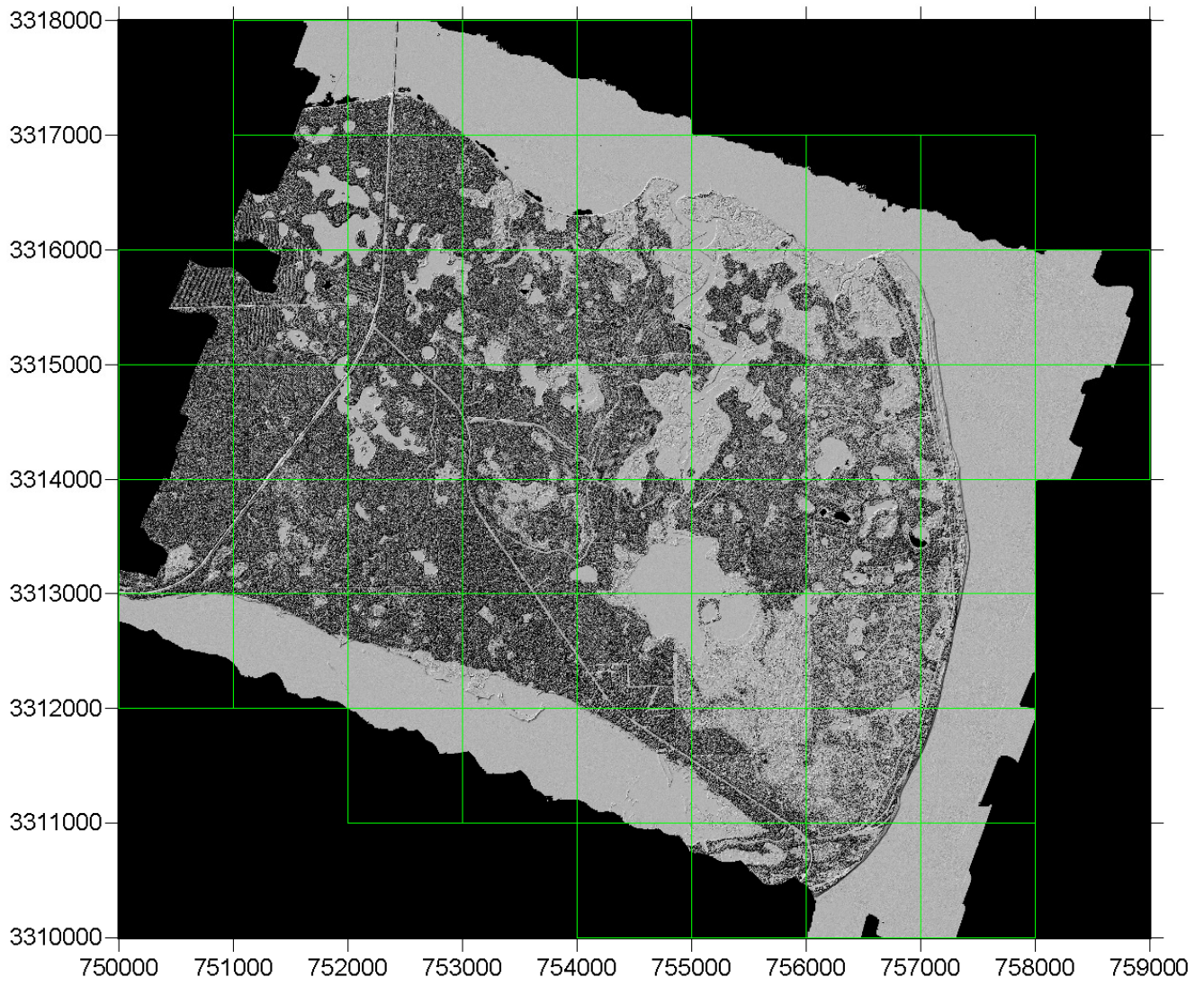
Figure 7 – Shaded relief image of Default Grid overlaid with Tile footprints
